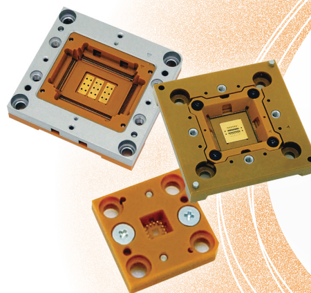
PACKAGE PROBE (TEST SOCKETS)
